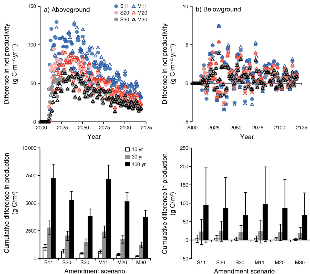
FIG. 5. Treatment differences averaged across site characterizations from control of (a) aboveground net primary production (ANPP) and (b) belowground net primary production (BNPP) for amendment scenarios are shown in the top row. In the bottom row, cumulative changes in ANPP and BNPP are shown over 10-, 30-, and 100-yr time periods. S indicates a single application of composted green waste (14.27 Mg C/ha). M indicates multiple annual applications of composted green waste (1.427 Mg C·ha -1 ·yr -1 for 10 consecutive years). The numbers next to S or M indicate C:N ratios, with 11 being a C:N ratio of 11.1, 20 indicating a C:N ratio of 20, and 30 indicating a C:N ratio of 30. Values above zero indicate greater aboveground C in amendment scenario vs. control.
