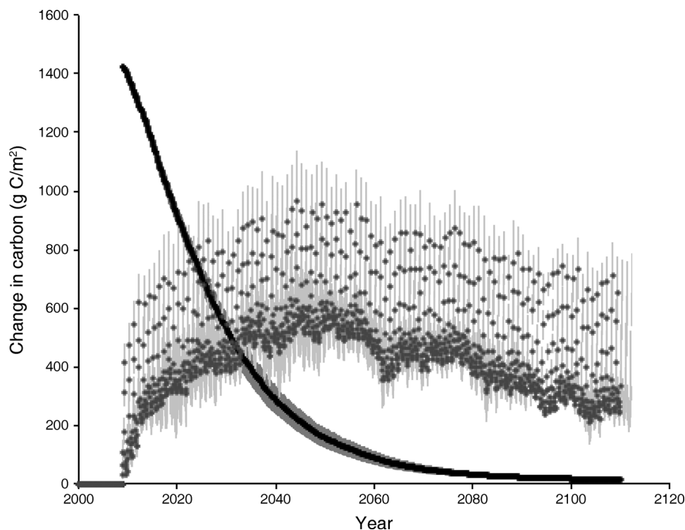
FIG. 3. The black line shows simulated decomposition of the composted organic matter amendment following application to grassland soils (site means \pm SD; y = 3 \times 10^{42}e^{-0.045x} ; r^2 = 0.99 ). Gray circles show the monthly change in total ecosystem carbon, not including compost carbon, in the S11 simulation. Values are averages across site characterizations, with standard error bars in light gray.
