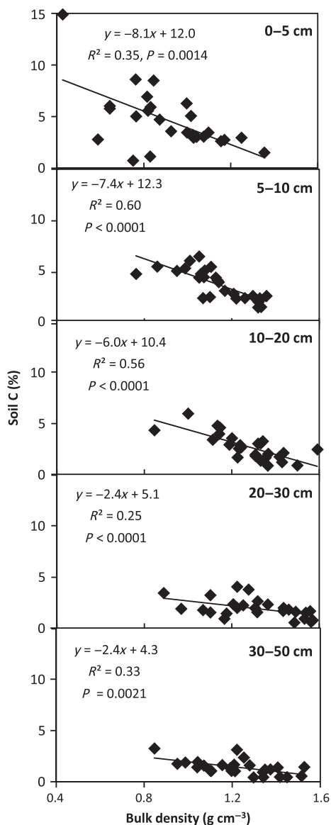
Fig. 4 Bulk density and soil C concentration by sample interval (in cm). All correlations are significant.
