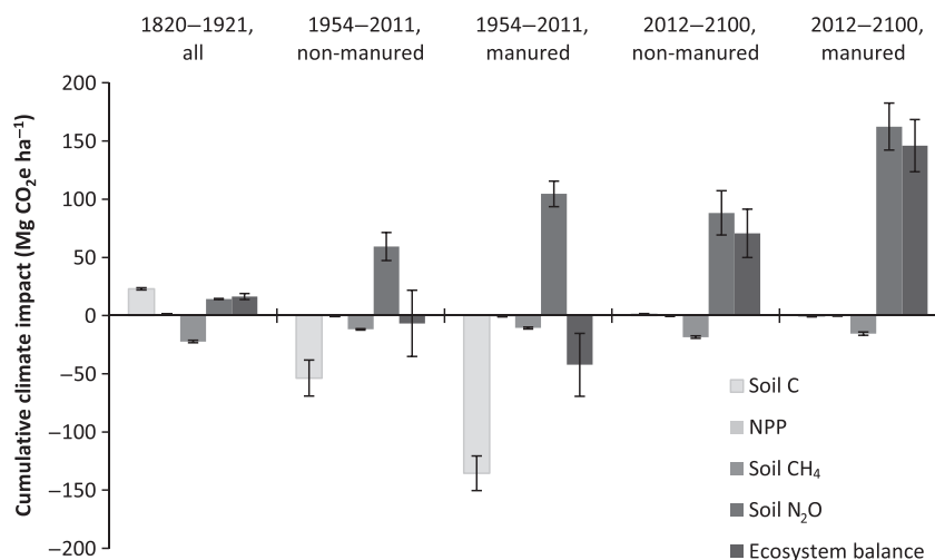
Fig. 11 The mean ( \pm standard error) cumulative climate impacts of soil greenhouse gas emissions, changes in soil C storage and NPP, and the net climate impact from 1820 to 1921, 1954 to 2011, and 2012 to 2100 for nonmanured and manured fields. These timespans represent the changes due to the shift in vegetation from perennial to annual grasses, intensive management of the past 60 years, and continued intensive management, respectively.
