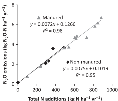
Fig. 10 Nitrous oxide emissions vs. total N additions (sum of N from fertilizer and manure) by field for the period 1954 to 2011.
