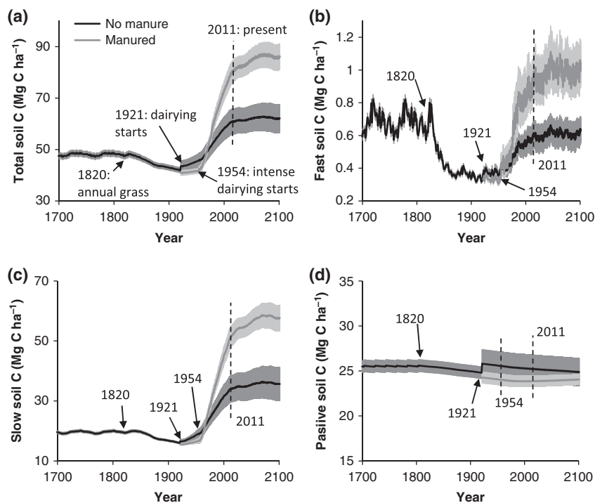
Fig. 6 Modeled soil C content for (a) total C, (b) fast pool, (c) slow pool, and (d) passive pool. Shaded areas around the data lines are standard errors. Vertical dashed lines denote years with important changes to management parameters. The apparently abrupt split in passive soil C pools (d) between manured and nonmanured fields in 1921 is an artifact of the model parameterization and data analysis.
