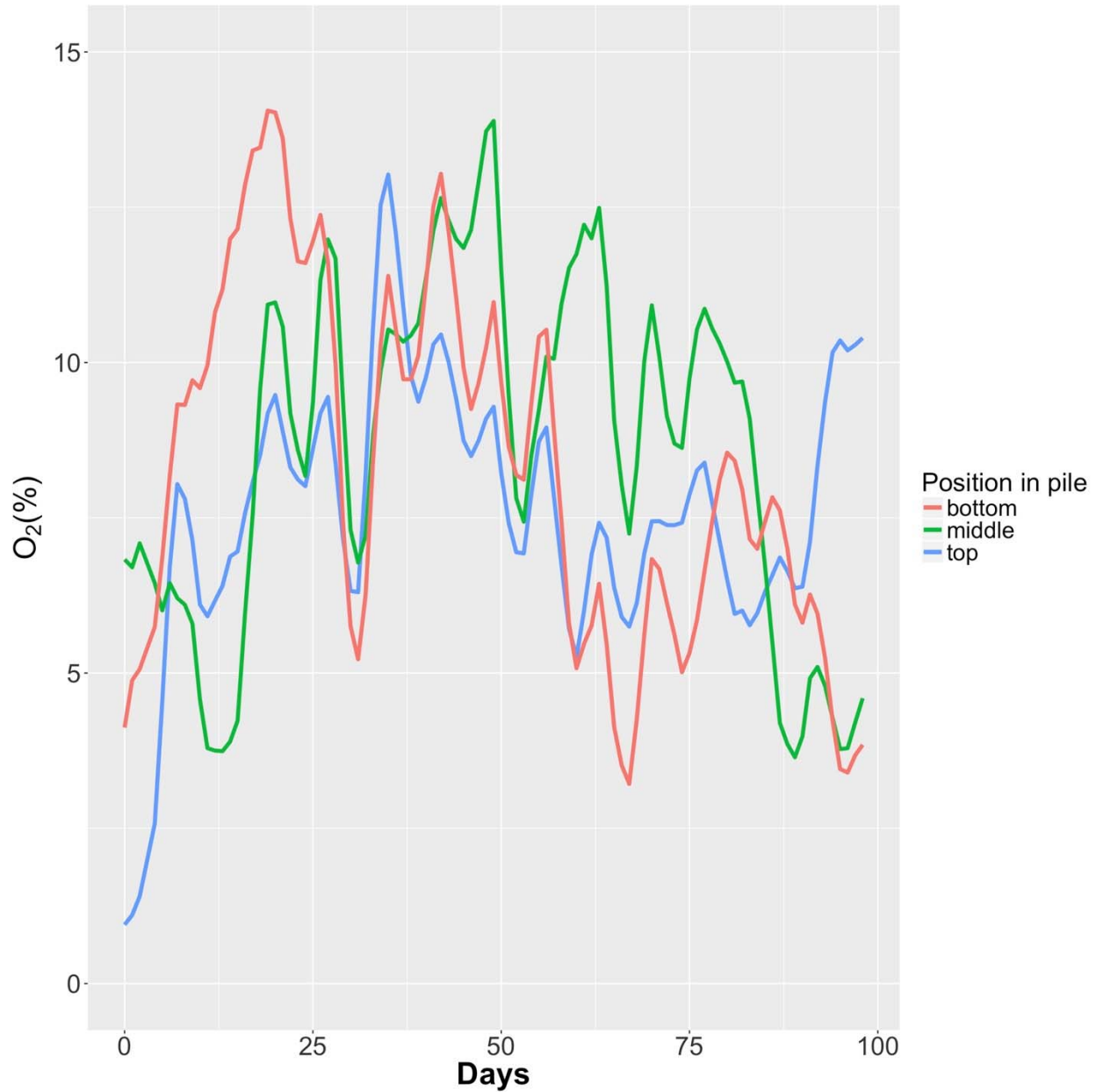
Figure 4.3: Oxygen concentrations within the composting pile show an inverted "U" shape over time. Pile 2.
