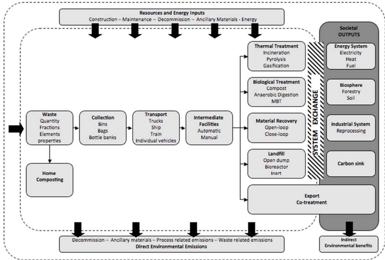
Figure 5.1: System boundary for waste management life cycle assessment (Vergara et al. 2011).
