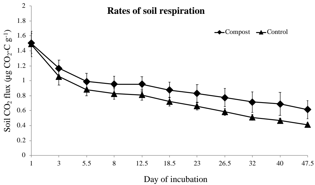
Figure 2.5: Rates of soil respiration during laboratory incubations of soils from the Santa Barbara County rangeland site. Data from Marchus and Schimel et al. in prep.
